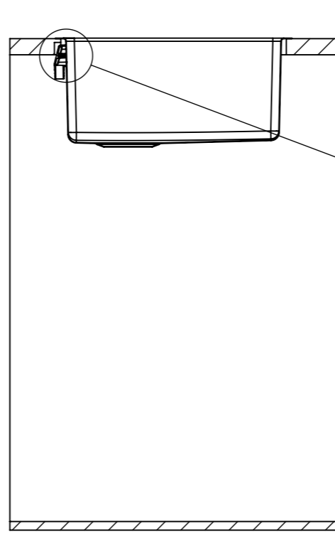
SECTION Z-Z
